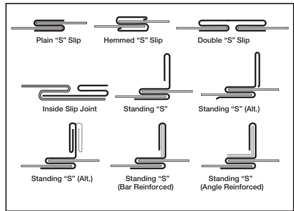
Figure 16 - Transverse Joints
