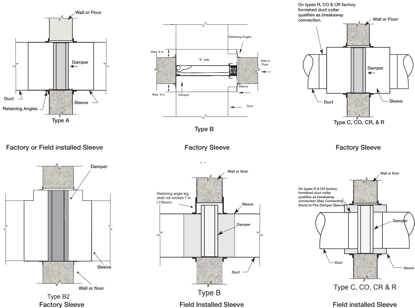
Figure 15: Damper/Sleeves with Transition
