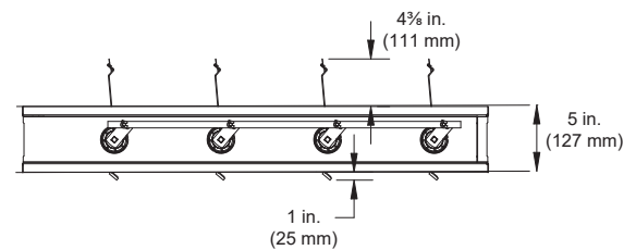
BR-10 No Flange
