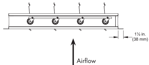
BR-12 Flange on Intake
