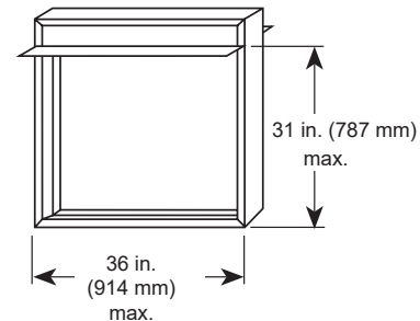
Type B Single Section
