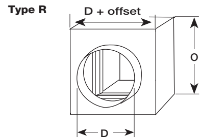
Overall Damper Dimensions
