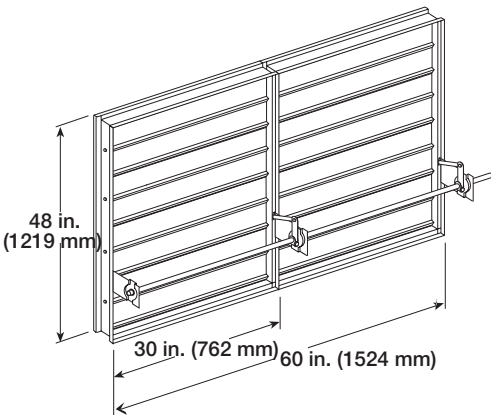
Two Section
