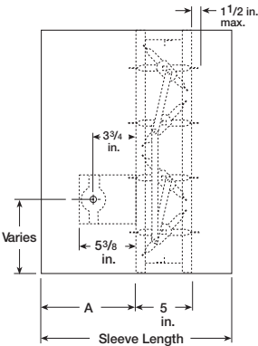
Sleeve
