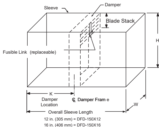
VERTICAL MOUNT
