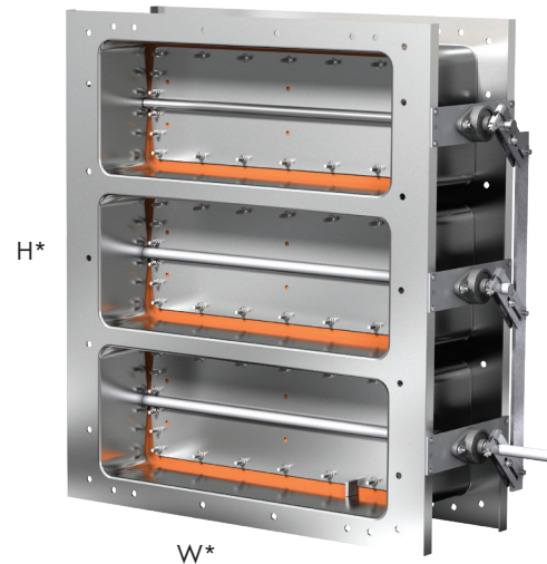
* Actual inside dimension. The W dimension is ALWAYS parallel with the damper blade length.
