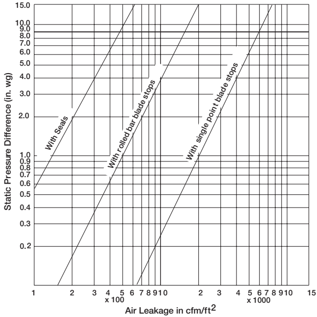
12 in. Diameter Damper
