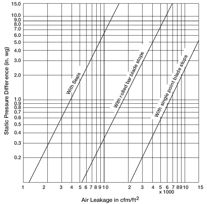
36 in. Diameter Damper
