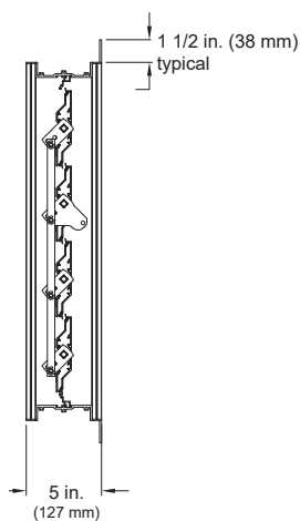
Reverse Flange
