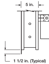
Reversed Flange
