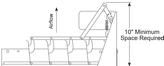
WD-100 backdraft damper with optional motorpack
